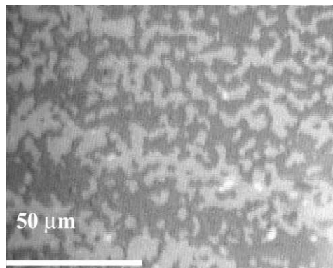
Fig. 4. Optical microscopy image of the surface topography of a BE37 film spin-coated from 2% DCM solution (sample D). Molten state at T=90^\circ\text{C} with terrace-like height variations.
