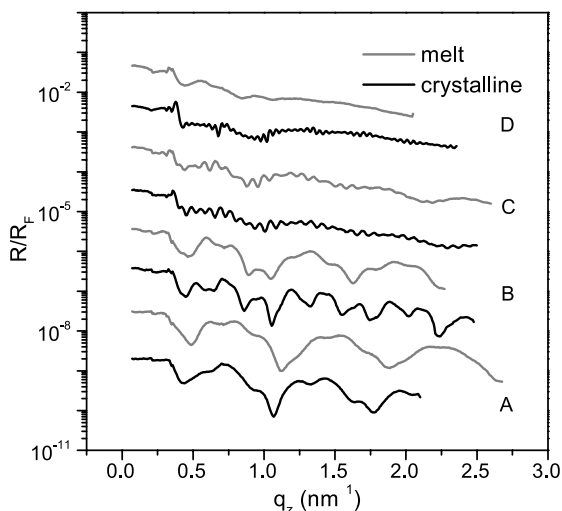
Fig. 6. Pairs of specular X-ray reflectivity curves of BE37 thin films at 90^\circ\text{C} (melt) and 35^\circ\text{C} (crystalline), respectively. A, B, C, D indicate the sample in increasing thickness. The curves are shifted for clarity.
