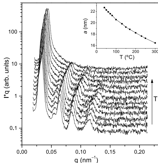
Fig. 1. SAXS profiles of BE37 in molten state at various temperatures (from bottom to top: 40\text{--}80 (with 10\text{ }^{\circ}\text{C} step), 100, 130, 150, 170, 200, 250, 300\text{ }^{\circ}\text{C} ). The curves are shifted for clarity and indicate hexagonal symmetry. The inset presents the hexagonal lattice parameter a=4\pi/(3^{1/2}q_{100}) as a function of temperature.
