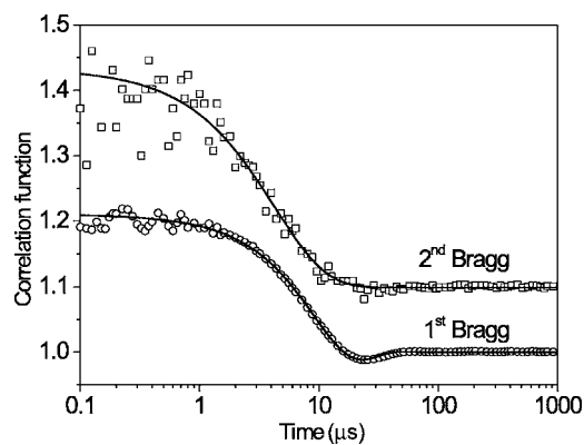
FIG. 8. Correlation functions measured at the first and second Bragg positions of a 13.2\text{-}\mu\text{m} -thick FPP membrane.
