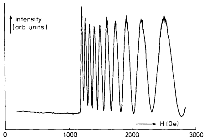
FIGURE 2 Interference pattern of a uniform planar nematic layer between crossed polarizers in monochromatic light (PAA, 131°C, d = 47.7 \mu\text{m} ).
