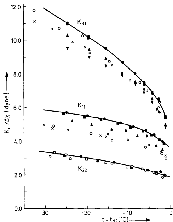
FIGURE 5 Elastic constants K_{ii}/\Delta\chi for PAA. ○ Tsvetkov (Ref. 3), × Saupe (Ref. 4), □ Madhusudana et al. (Ref. 11), Filled symbols: this work, surface treatments: ● K_{33} : 1-dodecanol, ■ K_{22} , K_{11} : polymer film + rubbing, ▲ K_{33} : chromic/sulphuric acid, ◻ K_{11} : rubbing + cremophor O, ▼ K_{33} : CTAB.
