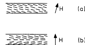
FIGURE 4 The two possible director patterns if the boundary conditions are not exactly tangential.
