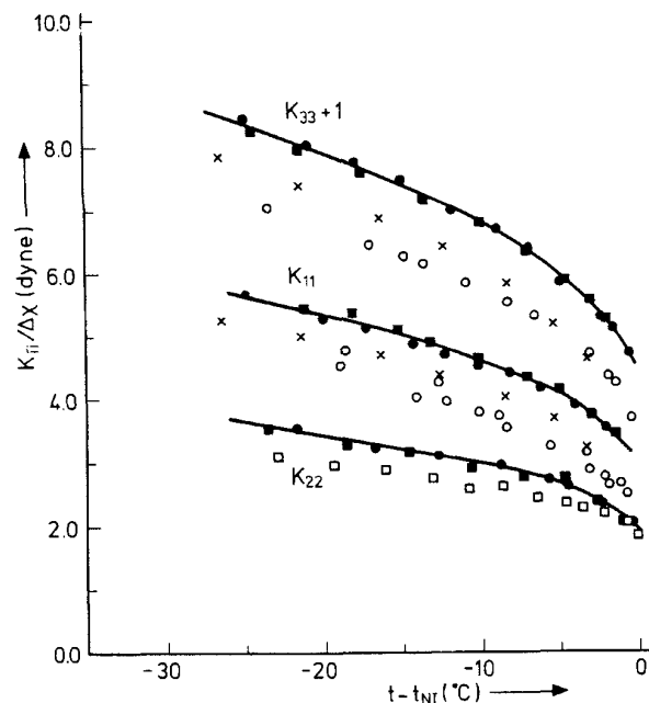
FIGURE 6 Elastic constants K_{ii}/\Delta\chi for MBBA. ○ Haller (Ref. 5), × Greulich et al. (Ref. 7), □ Leenhouts et al. (Ref. 17), Filled symbols: this work.
