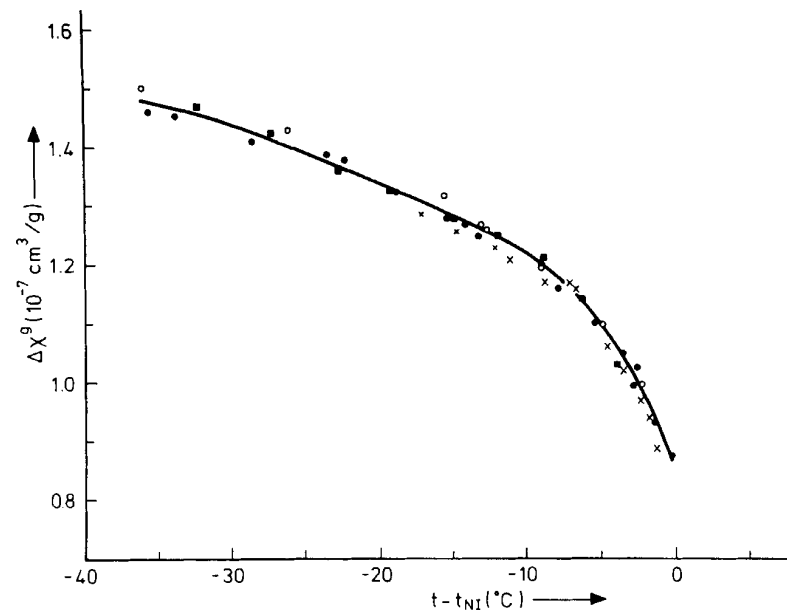
FIGURE 7 Diamagnetic anisotropy of PAA. ○ Foëx (Ref. 18), × Gasparoux et al. (Ref. 19), ●■ this work.
