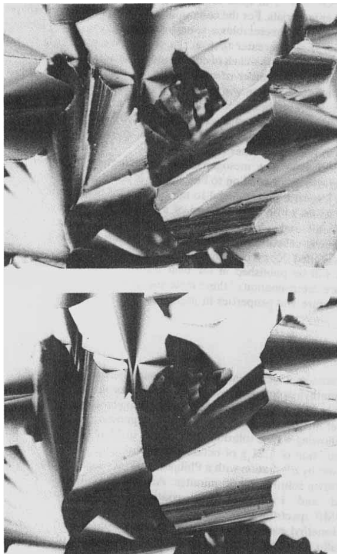
FIGURE 1 Textures, between crossed polars, of the D_{ha} phase at 180°C (a) and the D_{10} phase at 110°C (b) of [7]pizzane[10] ( n = 7 ).
