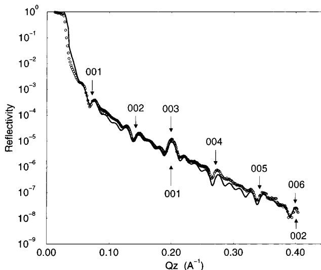
Figure 6. X-ray reflectivity of the diblock film after annealing in the SmA phase at T = 63 °C (circles) and the possible fitting curve (solid line) discussed in the text. The Bragg positions (00 l ) of the diblock periodicity (above the curve) and of the smectic spacing (below the curve) are indicated.
